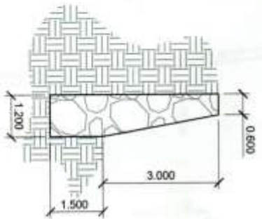
STONE MASONRY 1
