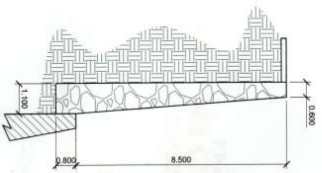
STONE MASONRY 4 PARAPETS
