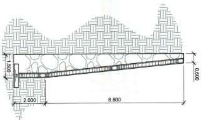
STONE MASONRY 1
