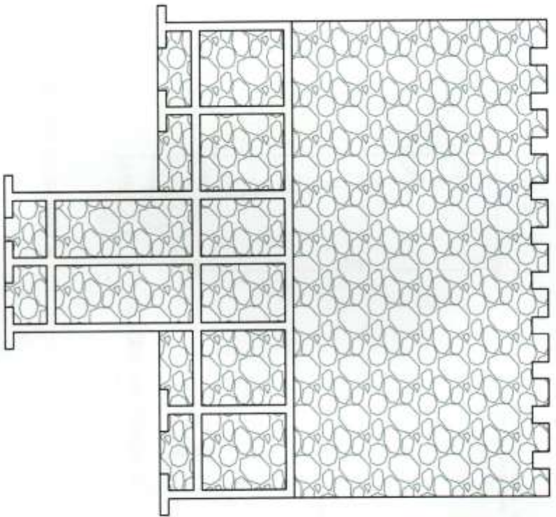
STONE MASONRY 1
